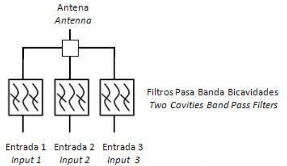
CONFIGURACIÓN TRIPLEXOR STAR-POINT STAR-POINT COMBINER CONFIGURATION
